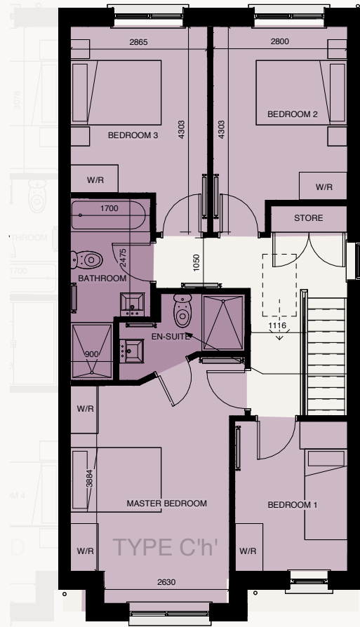
2 FIRST FLOOR
