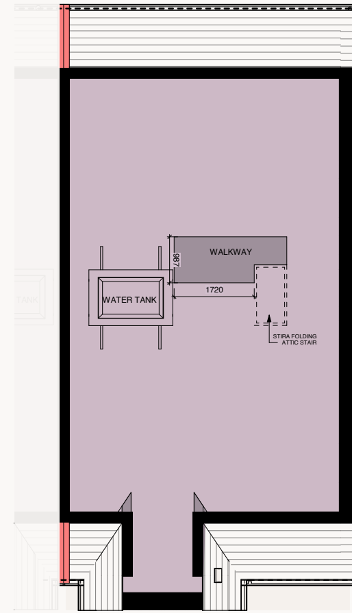
1 ATTIC PLAN
