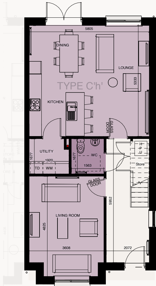
1 GROUND FLOOR
