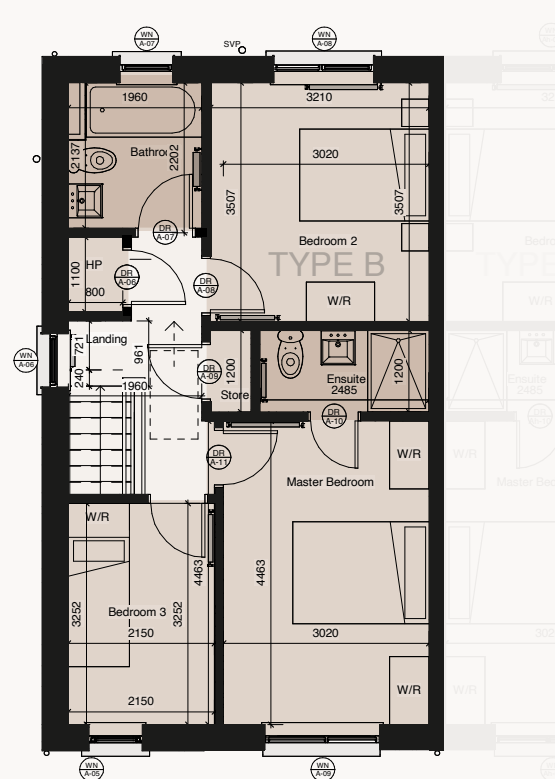
2 First Floor Plan - GA
