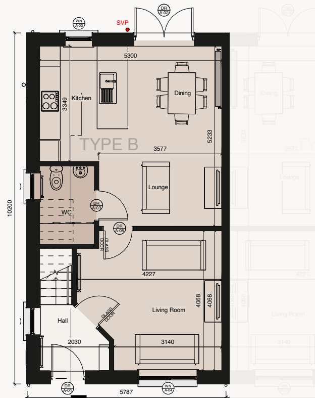
1 Ground Floor Plan - GA
